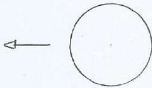
Planeta v = 30 \text{ km/s}
